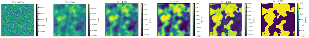
Snapshots of the spatial distribution of the spectator field \chi . The plots are order in increasing time from left to right. 5
