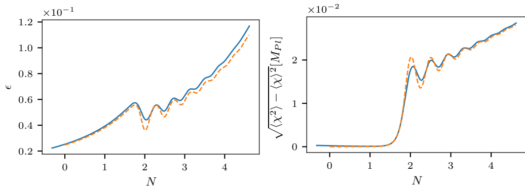
Evolution of the slow roll parameter \epsilon (left panel) and of the standard deviation of \chi (right panel). 5
